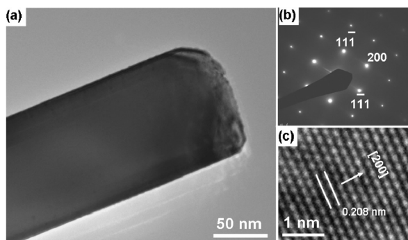
Figure 2. (a) Low resolution TEM image of a NiO NW. (b) SAED pattern and (c) HRTEM image taken on the same NW. The inter-plane distance of 0.208 nm is consistent with the lattice constant of NiO.
